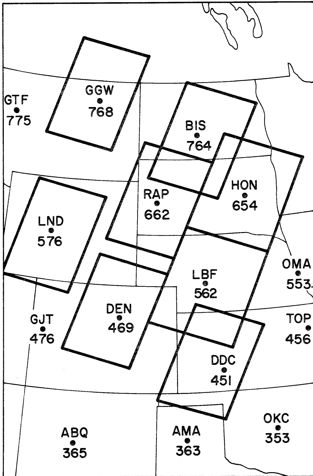
Figure 13. Radiosonde-Satellite Mesoscale Fields 9 August 1973 17 GMT
