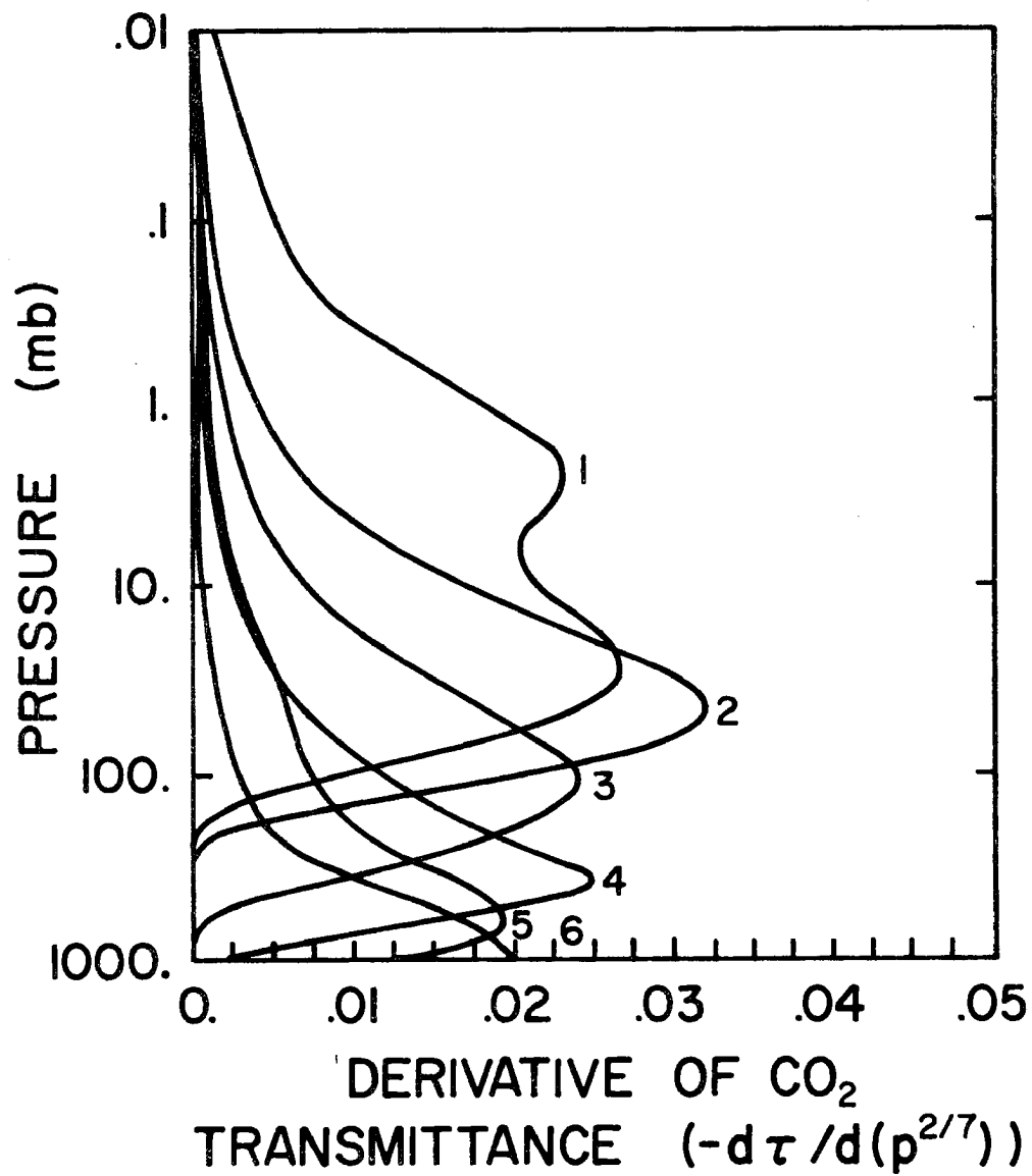
Figure 3. VTPR CO 2 Channel Weighting Functions for US Standard Atmosphere
