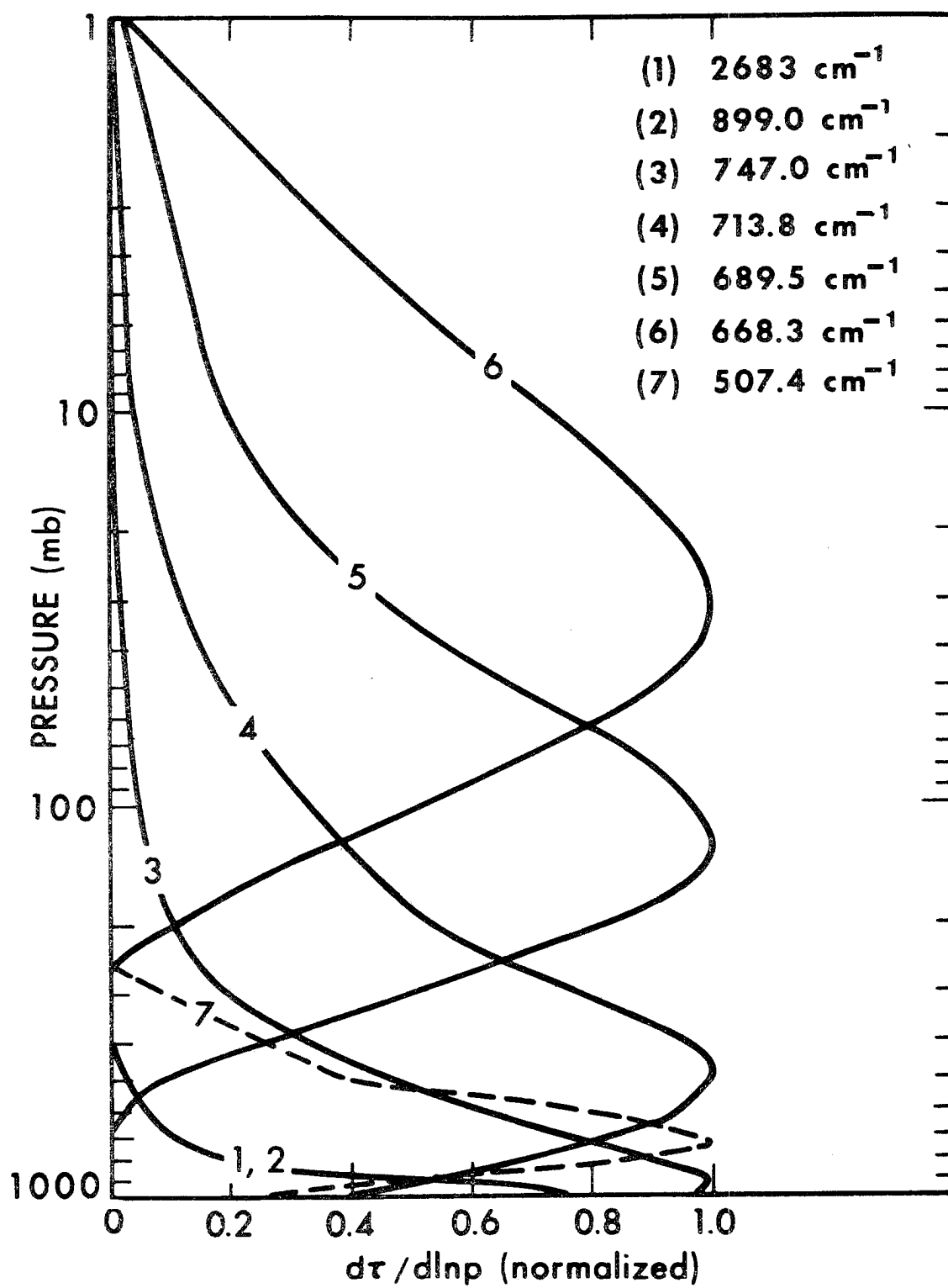
Figure 6. ITPR Weighting Functions (Nimbus-5 User's Guide)
