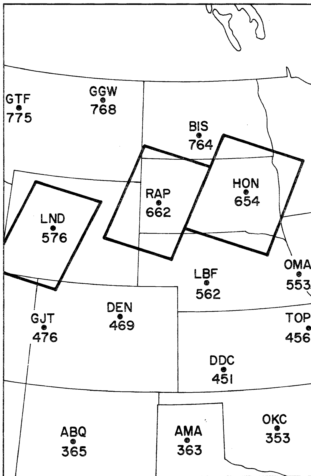
Figure 12. Radiosonde-Satellite Mesoscale Fields 7 August 1973 17 GMT
