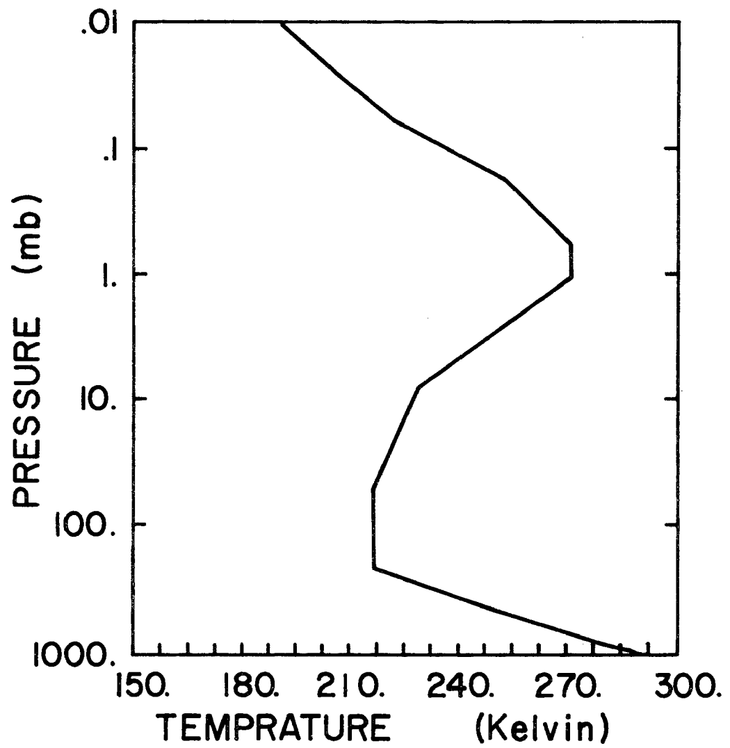
Figure 4. Standard Atmosphere Supplement Mid-latitude Spring-Fall
