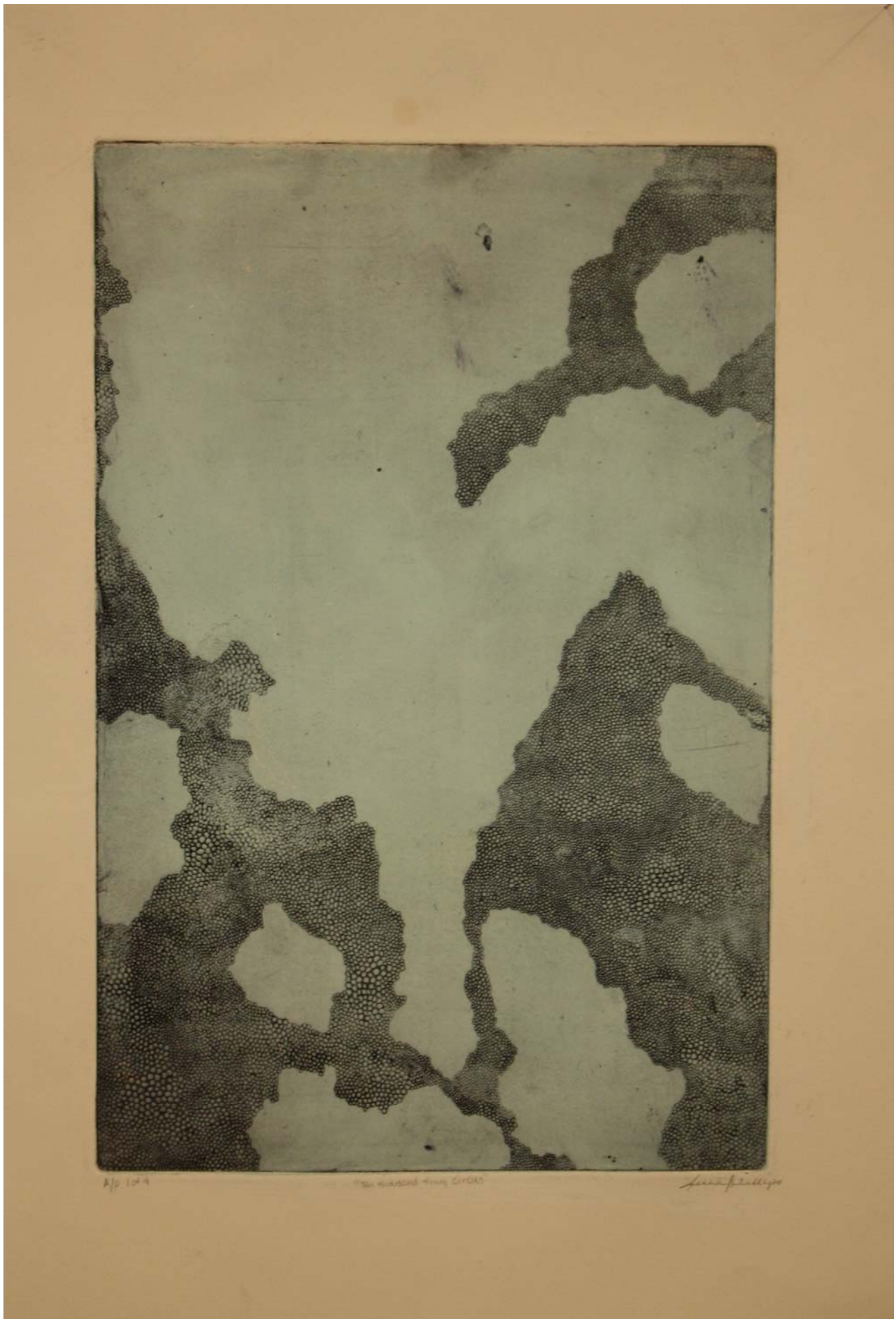
Figure 5: Ten Thousand Tiny Circles.
