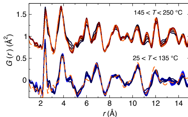
Figure 4.5: PDF analysis of the synchrotron PXRD data. No major changes in the local structure occur below 145 °C, which suggests that the intermediate structures have close relationships to one another. At these lower temperatures, the phases NaCl, CuSe, pyrite \text{CuSe}_2 provide a reasonable description of the local structure, whereas NaCl, marcasite, pyrite, and CuSe are found at the higher temperatures. At the shortest distances ( r 2.2~2.3 Å), there is some intensity in G(r) that is not accounted for by the calculated patterns, which suggests the presence of some poorly-ordered or amorphous components. (fit curve: dashed orange lines; higher temperature data offset for clarity).
