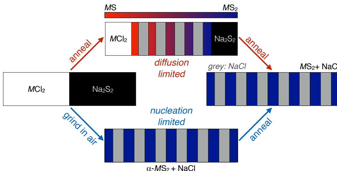
Figure 3.6: Scheme illustrating the different observed reaction pathways of the metathesis reactions. Preparing the reactants in a strictly air-free and anhydrous manner leads to a diffusion-limited reaction which in turn allows the formation of a range of MS_x phases ( x \leq 2 ). Grinding the reactants in air allows NaCl formation along with an amorphous ( \alpha ) material of the nominal composition MS_2 . Annealing leads to direct nucleation of the crystalline MS_2 phase.
