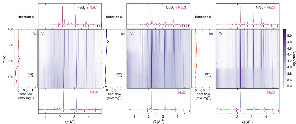
Figure 3.3: In situ DSC [(a), (c), (e)] and SXR D [(b), (d), (f)] of the air-exposed solid state metathesis reactions of MCl_2 + Na_2S_2 \rightarrow MS_2 + 2 NaCl , M = Fe (Reaction 4), Co (Reaction 5), and Ni (Reaction 6), respectively. In the air exposed reactions, the reaction pathway is extensively altered compared to the air-free reactions, with NaCl present throughout and no apparent crystalline intermediates, the products instead crystallizing out of the reaction mixtures. There are significant diffuse features in the background as well, indicating the presence of an amorphous phase. This is especially apparent in 5 and 6. The diffraction patterns of the as-prepared reactants and the products at 400 °C are shown below and above each color plot, respectively.
