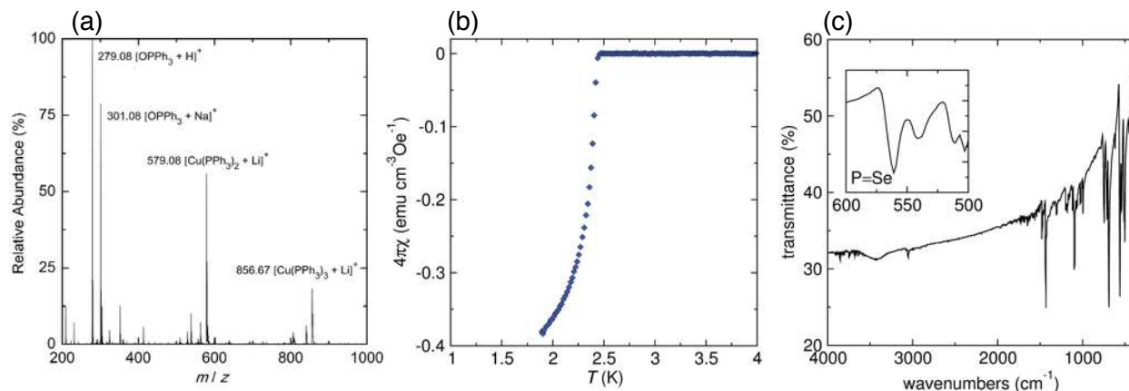
Figure 5.2: (a) Mass spectrum of \text{CuCl}_2 + \text{Na}_2\text{Se}_2 + 0.1 \text{ Ph}_3\text{P} reacted at 130^\circ\text{C} for 96 hours with intermittent grinding every 24 hours, performed in \text{CH}_3\text{OH} with the four most intense peaks labelled. The triphenylphosphine oxide formation is a result of the conditions used to perform the experiment. (b) Measurement of magnetic susceptibility as a function of temperature indicates a transition to a superconducting state at T_c = 2.4 \text{ K} in a sample of \text{CuSe}_2 produced from \text{CuCl}_2 + \text{Na}_2\text{Se}_2 + 0.1 \text{ Ph}_3\text{P} reacted at 150^\circ\text{C} for 24 hours, then washed 5 times each with benzene and methanol. (c) IR spectrum of the products of \text{CuCl}_2 + \text{Na}_2\text{Se}_2 + 0.97 \text{ Ph}_3\text{P} . The inset shows the characteristic \text{P}=\text{Se} stretch at 560 \text{ cm}^{-1} , which is not present in either the \text{Ph}_3\text{P} or \text{Ph}_3\text{P}=\text{O} spectra.
