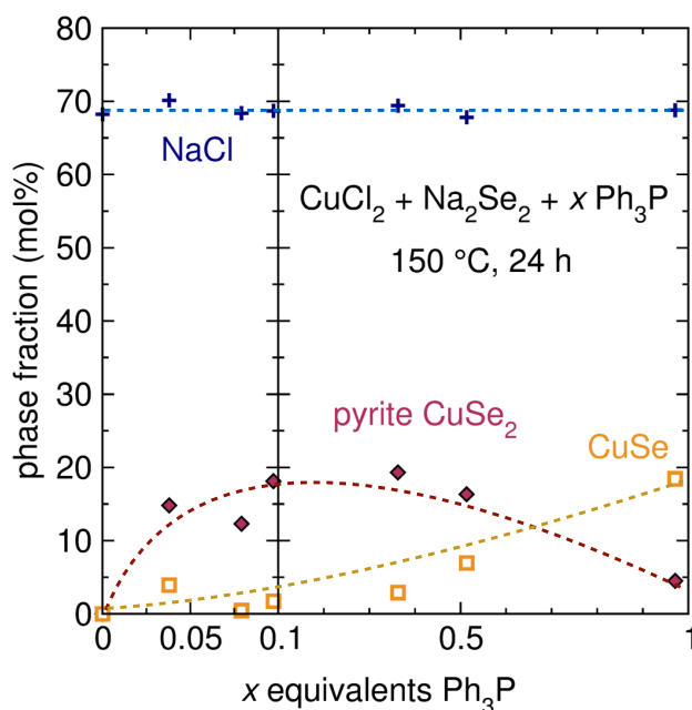
Figure 5.4: Molar phase fractions of NaCl, \text{CuSe}_2 , and CuSe extracted from the Rietveld refinements of PXRD patterns of the products of \text{CuCl}_2 + \text{Na}_2\text{Se}_2 + x \text{Ph}_3\text{P} after 24 hours at 150 °C. Adding more than \approx 10\% \text{Ph}_3\text{P} does not promote further pyrite formation, and at increased concentrations \text{Ph}_3\text{P} promotes CuSe formation rather than \text{CuSe}_2 . NaCl content remains relatively constant, and quantitative at \approx 67\% . Dashed lines serve as a guide to the eye. Phase fractions of CuCl and selenium are omitted for clarity. Note the split x-axis at x = 0.1 .
