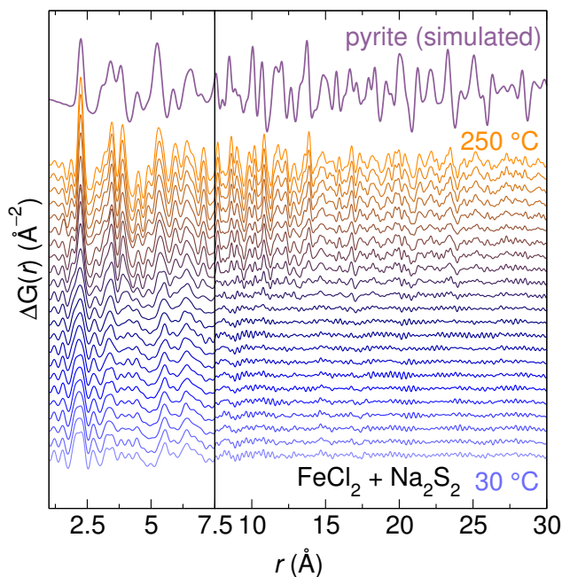
Figure 3.5: In situ differential PDF analysis of Reaction 4 ( FeCl_2 + Na_2S_2 ) with the pairwise correlations arising from NaCl subtracted. The differential PDF at lower temperatures reveals only short range correlations; longer range correlations consistent with crystallization gradually grow in starting around T \approx 160 °C, in agreement with in situ PXRD data. The high temperature differential PDF is identical to that of pyrite FeS_2 . The offset data are taken in 10 °C increments.
