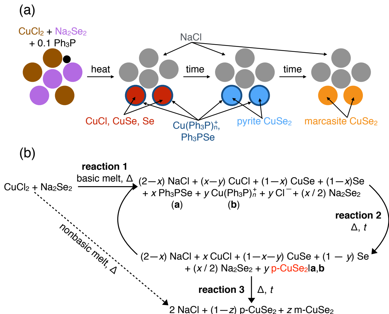
Figure 5.7: (a) A cartoon summarizing the polymorph-selective pathway of \text{CuSe}_2 formation, mediated by \text{Ph}_3\text{PSe} and \text{Cu(Ph}_3\text{P)}_n^+ . (b) The hypothesized reaction pathway yielding polymorph selectivity of \text{CuSe}_2 . Formation of a and b allow the stabilization of the pyrite polymorph before conversion to marcasite at longer reaction times. Without the addition of the Lewis base, no selectivity is observed and direct formation of marcasite occurs. (e.g., direct, dashed arrow)
