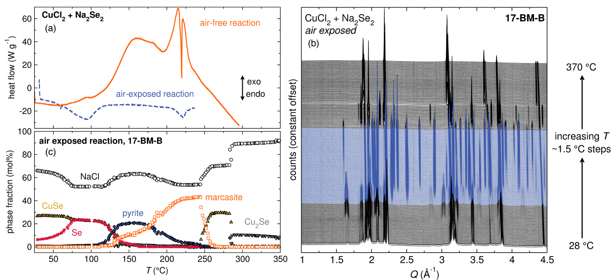
Figure 4.4: (a) DSC curves of the air-free (orange) and air-exposed (blue) reaction of CuCl_2 and Na_2Se_2 . (b) In situ SXRD data collected from the air-exposed reaction mixture, as heated under vacuum. (c) The extracted phase fractions from the Rietveld refinements of the in situ SXRD measurements of the air-exposed reaction.
