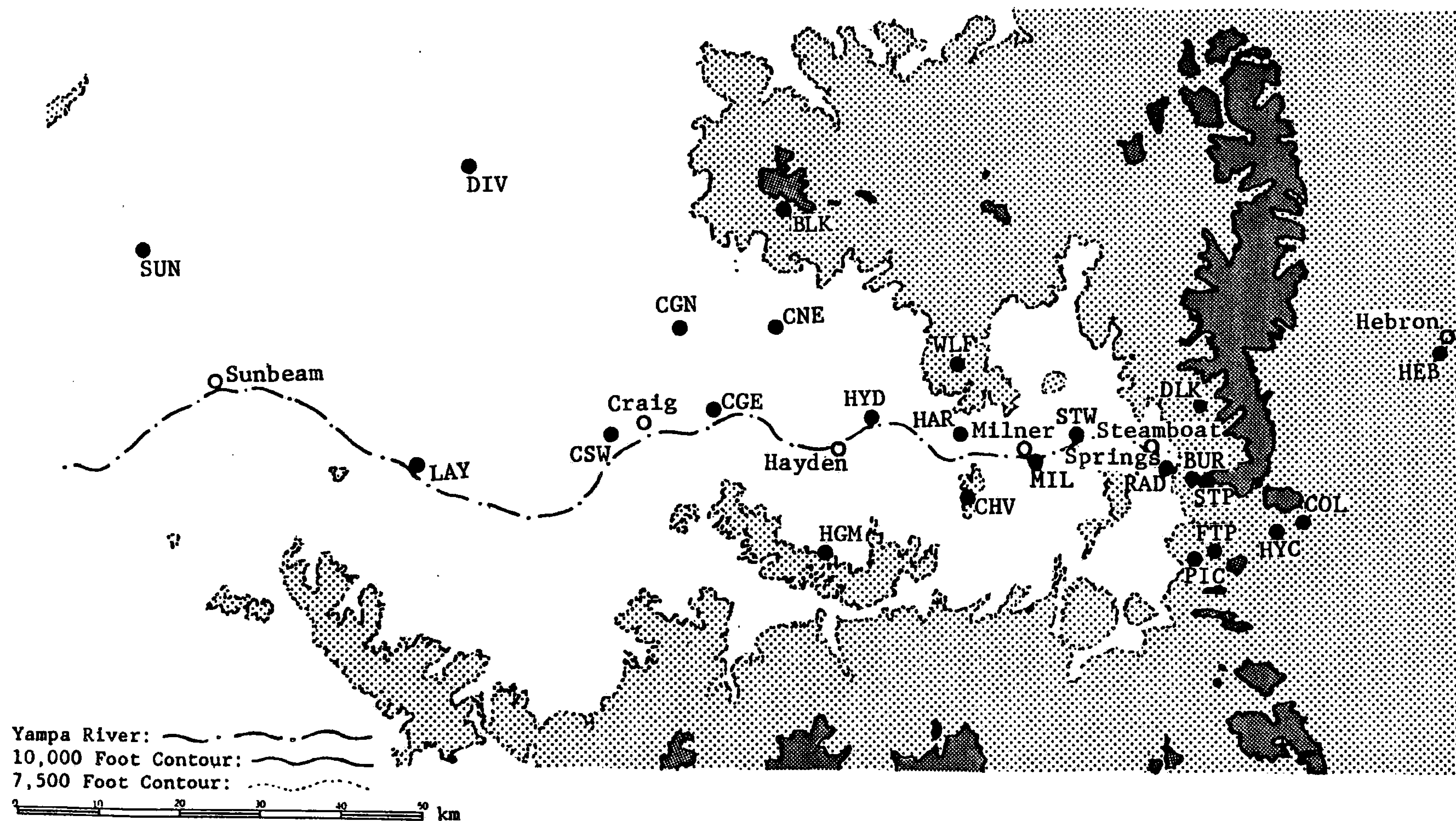
Figure 1. A map of the COSE III research area showing towns and PROBE station names and elevations. Lightly stippled area represents elevations between 7,500 feet and 10,000 feet MSL. Darker stippling represents elevations greater than 10,000 feet.
