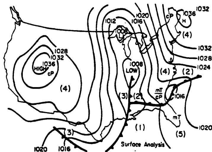
Figure 36. Example of Yu and Pielke's synoptic classification scheme. From Yu and Pielke (1986).
