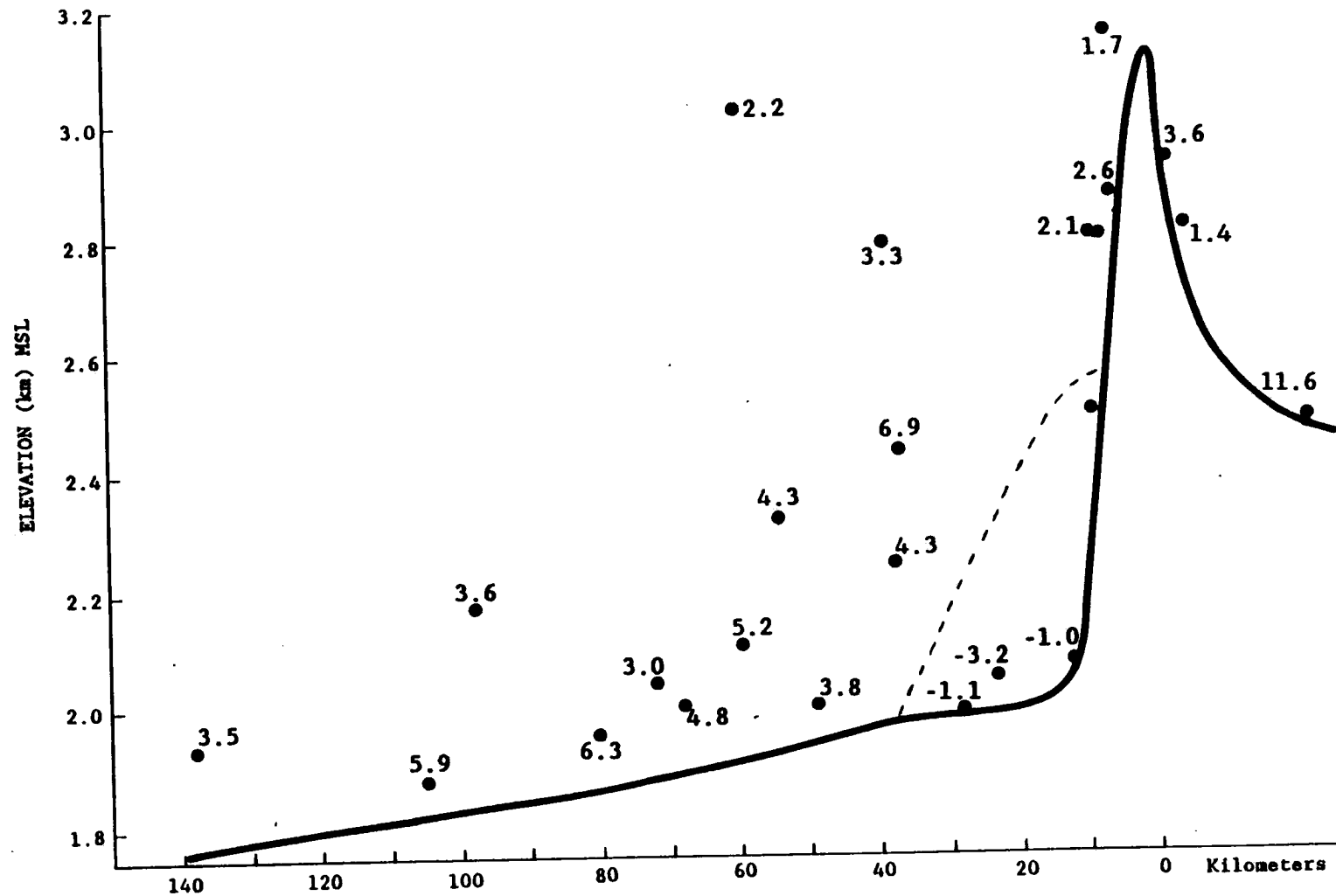
Figure 79. U-wind component from the PROBE stations plotted on a cross section of the research area, January 16, 1982 1930 GMT. The dashed line is the 1.0 ms -1 contour.
