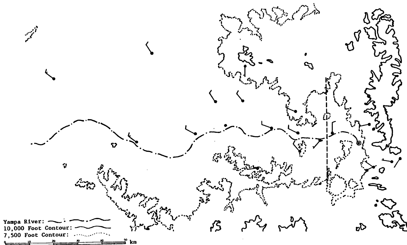
Figure 10. COSE III research area showing PROBE station wind barbs in knots. Heavy dashed line represents the westward extent of decoupled flow determined by the computer program. This example is for 26 km of decoupled flow from winds recorded December 13, 1981 at 22:00 GMT. Long wind barbs are 5 \text{ ms}^{-1} .
