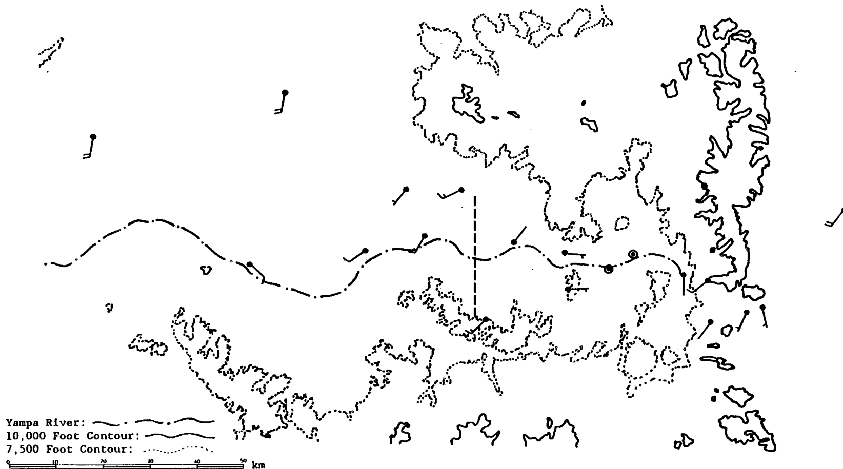
Figure 12. COSE III research area showing PROBE station wind barbs in knots. Heavy dashed line represents the westward extent of decoupled flow determined by the computer program. This example is for 58 km of decoupled flow from winds recorded January 5, 1982 at 10:00 GMT. Long wind barbs are 5 ms -1 .
