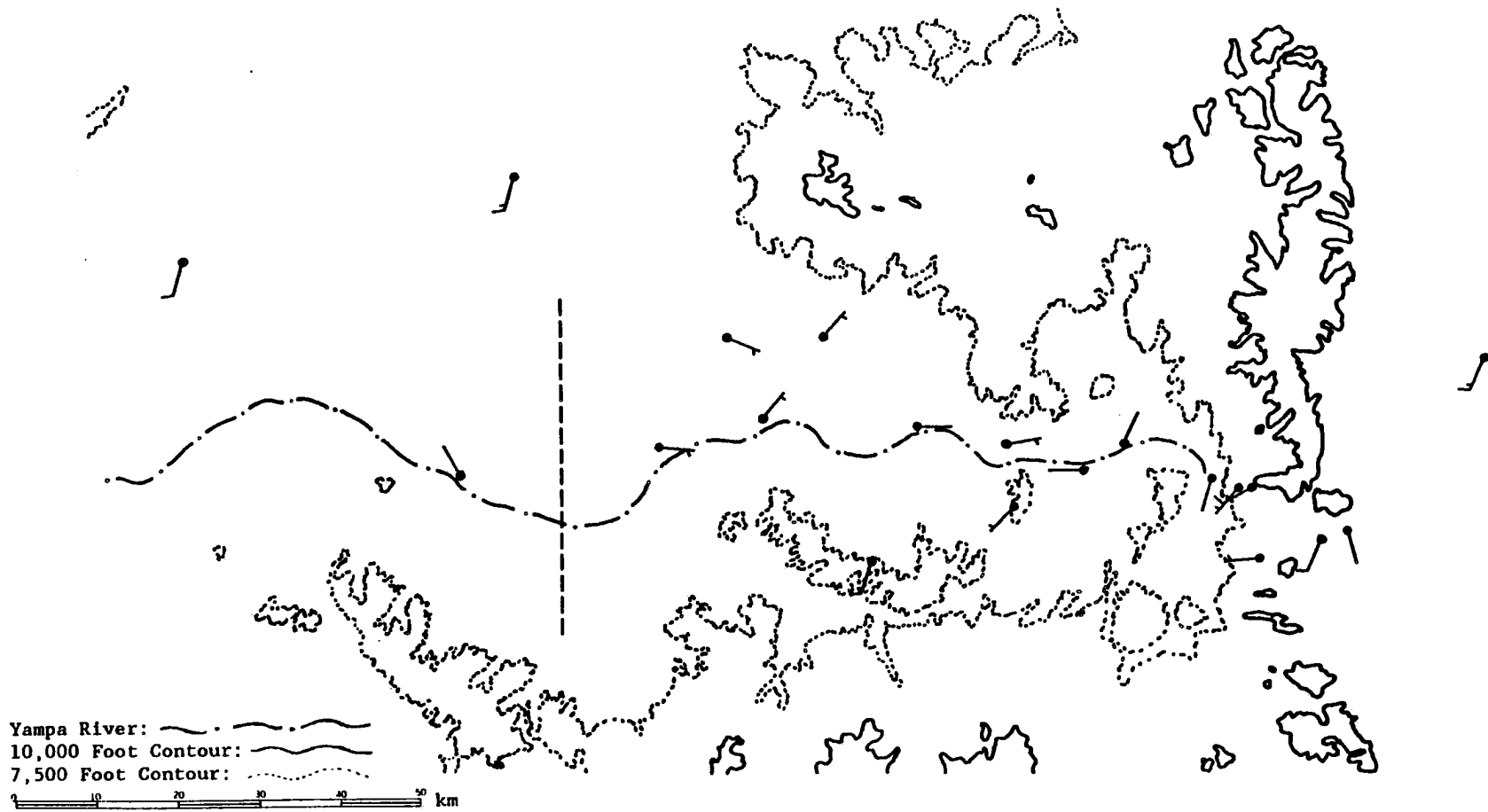
Figure 14. COSE III research area showing PROBE station wind barbs in knots. Heavy dashed line represents the westward extent of decoupled flow determined by the computer program. This example is for 92 km of decoupled flow from winds recorded January 5, 1982 at 19:00 GMT. Long wind barbs are 5 \text{ ms}^{-1} .
