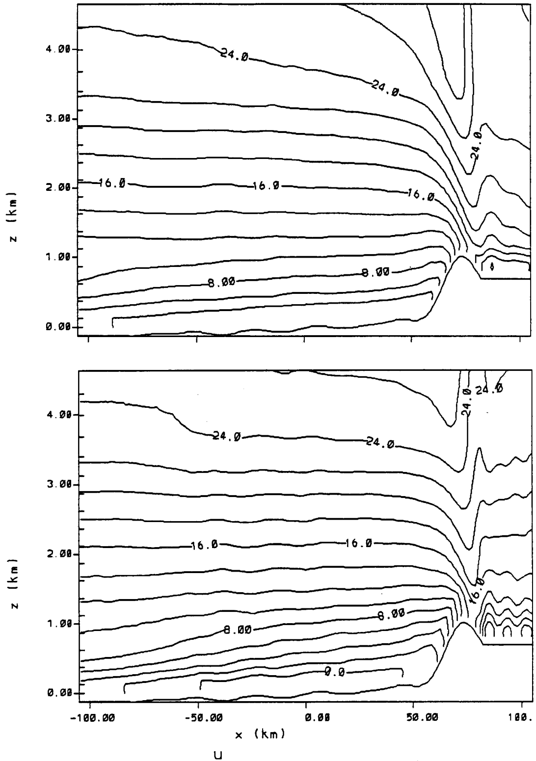
Figure 91. U-wind fields at 4 hours for the no decoupled flow case (top) and the decoupled flow case (bottom). Contour increment is 2 ms -1 .
