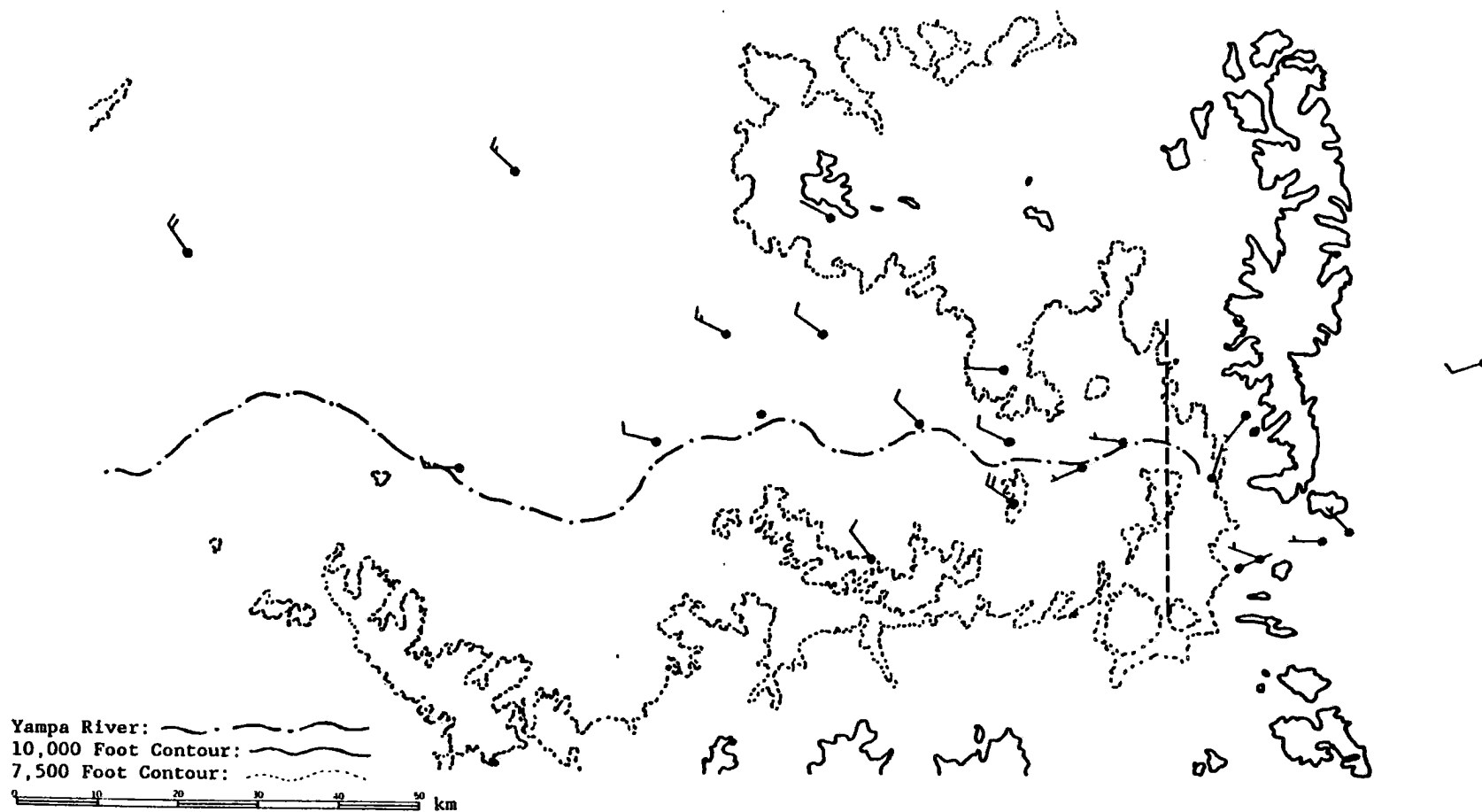
Figure 9. COSE III research area showing PROBE station wind barbs in knots. Heavy dashed line represents the westward extent of decoupled flow determined by the computer program. This example is for 18 km of decoupled flow from winds recorded December 13, 1981 at 20:00 GMT. Long wind barbs are 5 \text{ ms}^{-1} .
