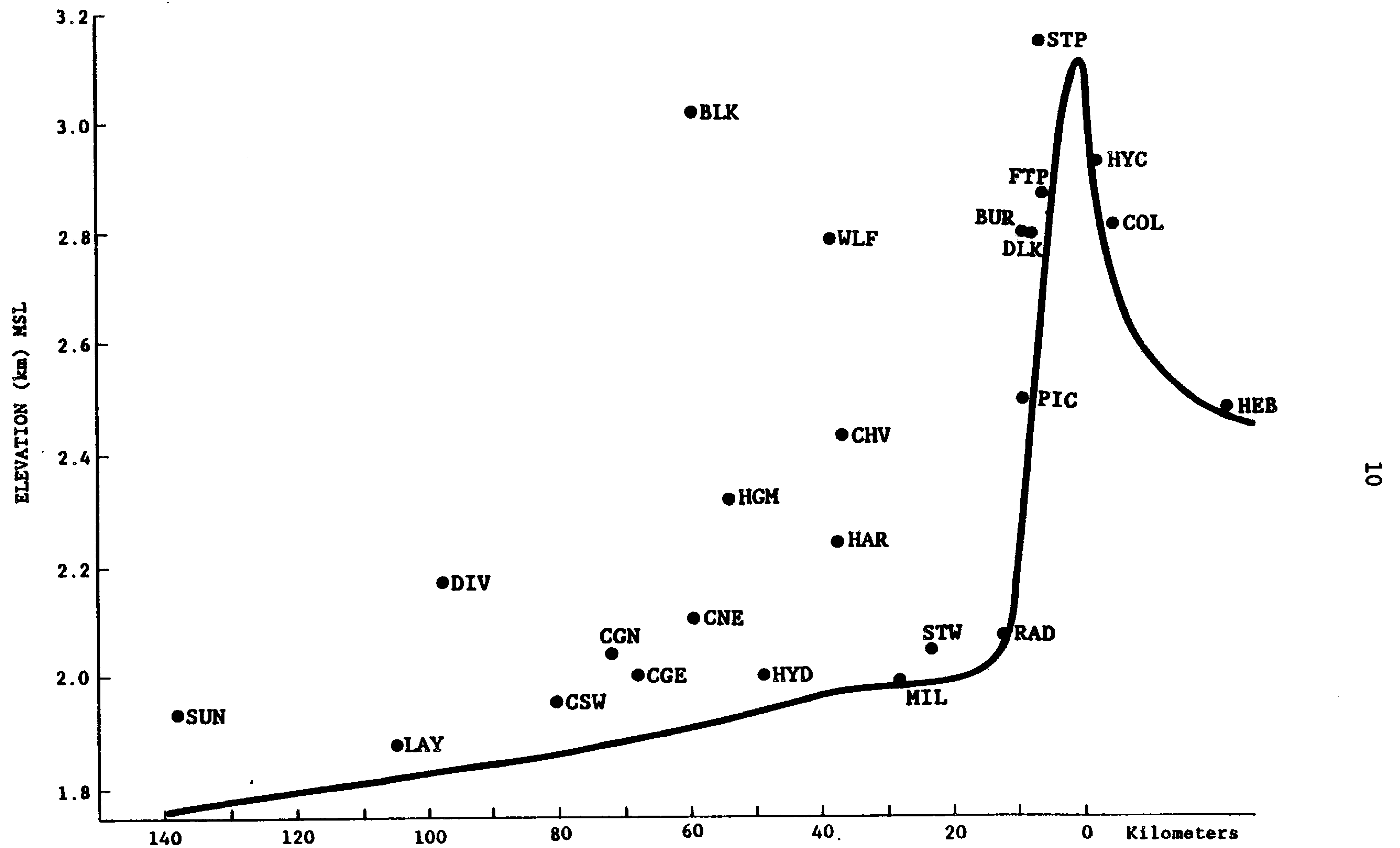
Figure 6. West-east cross section of the COSE III research area showing the name and location of PROBE stations in relation to the Yampa River valley floor elevation.
