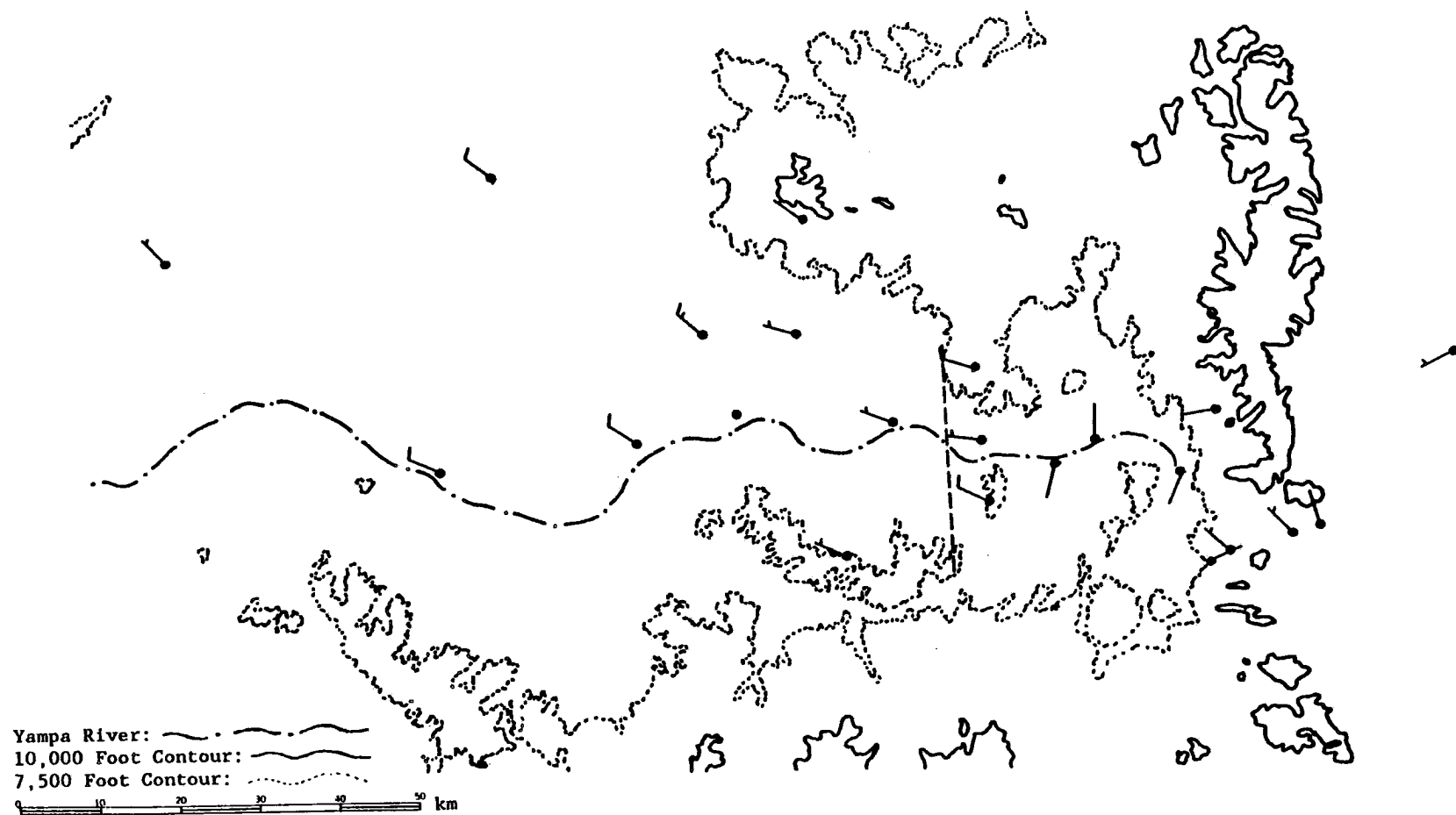
Figure 11. COSE III research area showing PROBE station wind barbs in knots. Heavy dashed line represents the westward extent of decoupled flow determined by the computer program. This example is for 38 km of decoupled flow from winds recorded December 14, 1981 at 00:00 GMT. Long wind barbs are 5 \text{ ms}^{-1} .
