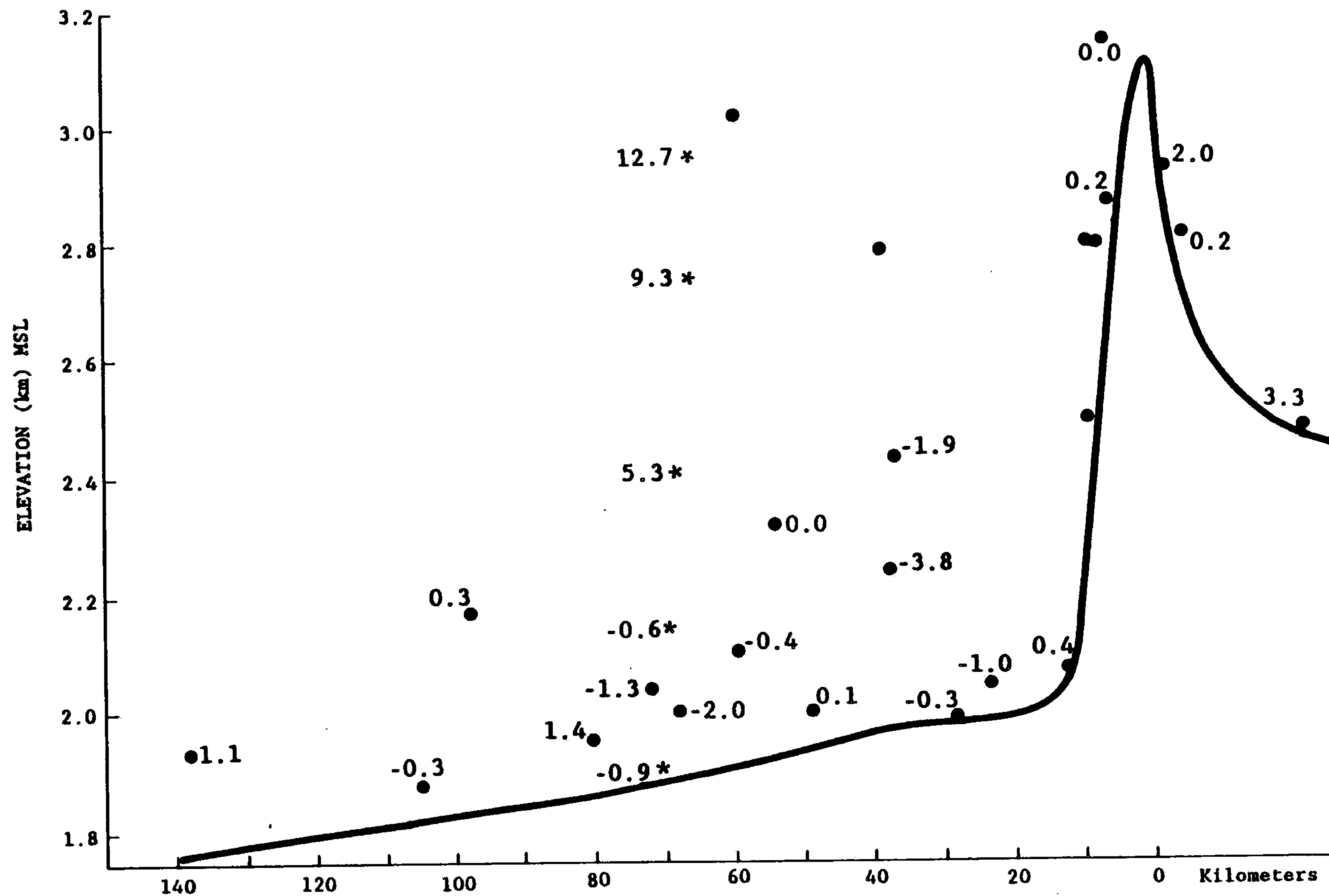
Figure 7. XZ cross section of COSE III research area with the cross-barrier wind component in m^{-1} recorded by PROBE stations (dots) and by a rawinsonde (stars) on January 5, 1982 15:00 GMT.
