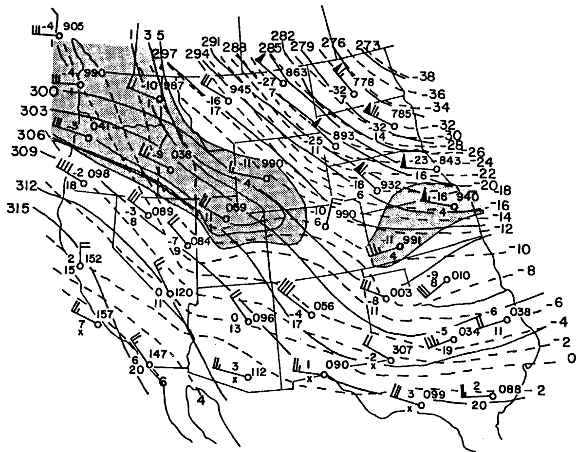
Figure 73. The 700 hPa analysis of height, temperature and dew point depressions ( T-T_d ) fields at 1200 GMT on January 16, 1982. The shaded area denotes region where T-T_d < 5^\circ\text{C} . Long wind barbs are 5 \text{ m s}^{-1} . Pennant barbs are 25 \text{ m s}^{-1} . From Rauber, 1987.
