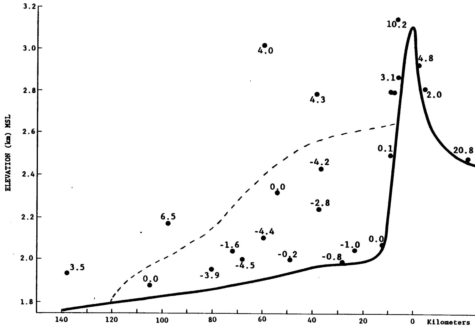
Figure 80. U-wind component from the PROBE stations plotted on a cross section of the Yampa Valley, January 23, 1982 2245 GMT. The dashed line is the 1.0 ms -1 contour.
