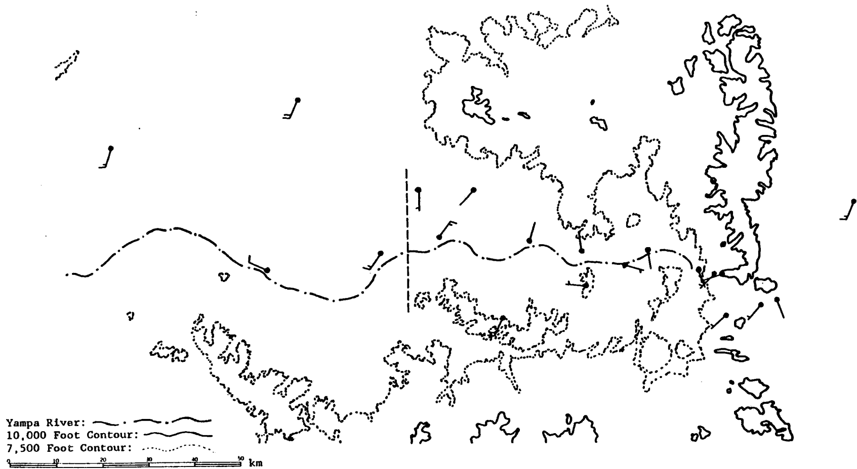
Figure 13. COSE III research area showing PROBE station wind barbs in knots. Heavy dashed line represents the westward extent of decoupled flow determined by the computer program. This example is for 74 km of decoupled flow from winds recorded January 5, 1982 at 20:00 GMT. Long wind barbs are 5 \text{ ms}^{-1} .
