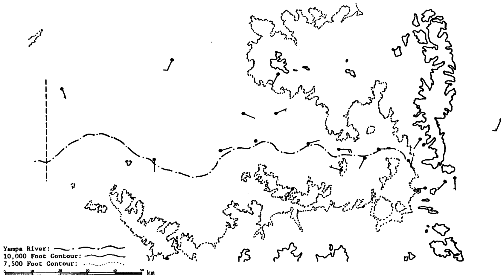
Figure 16. COSE III research area showing PROBE station wind barbs in knots. Heavy dashed line represents the westward extent of decoupled flow determined by the computer program. This example is for 140 km of decoupled flow from winds recorded December 14, 1981 at 12:00 GMT. Long wind barbs are 5 ms -1 .
