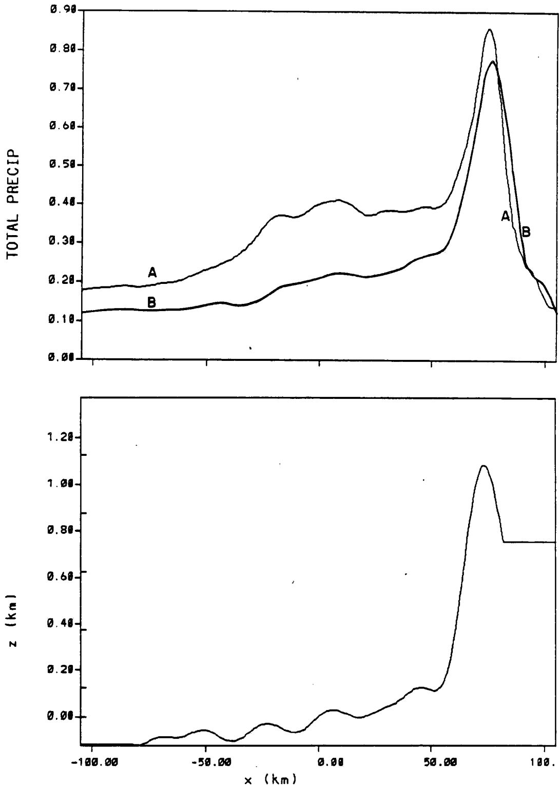
Figure 94. Total precipitation (top) at 4\frac{1}{2} hours ( 2\frac{1}{2} hours of full microphysics) for both the decoupled flow case (A) and the no decoupled flow case (B) in cm water equivalence. The bottom chart is the topography.
