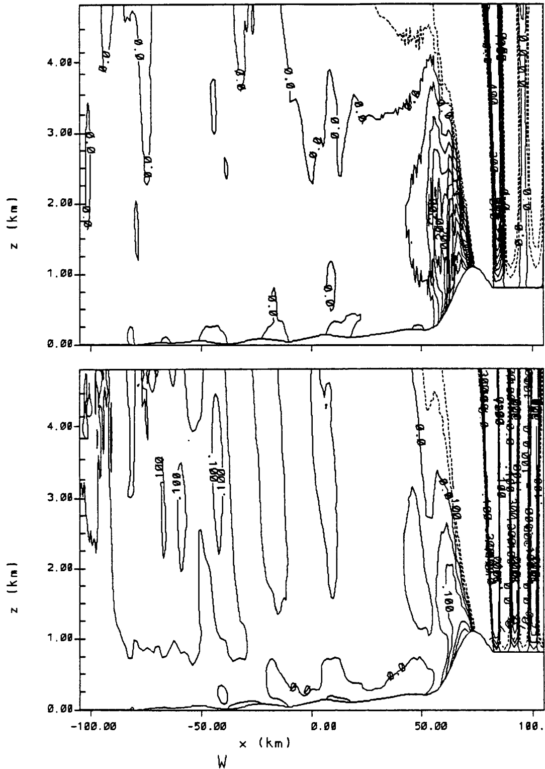
Figure 92. Vertical wind field at 4 hours for both the no decoupled flow case (top) and the decoupled flow case (bottom). The contour increment of 0.05 ms -1 was applied from -0.1 to 0.5 ms -1 .
