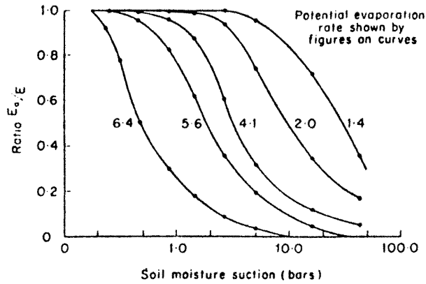
Figure 2.5a. Relative evapotranspiration as a function of soil moisture tension and rate of evapotranspiration (Withers and Vipond, 1974).
