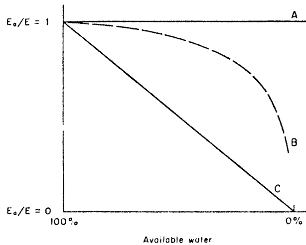
Figure 2.5b. Relative evapotranspiration as a function of available water for different theories of water availability to plants (Withers and Vipond, 1974).
