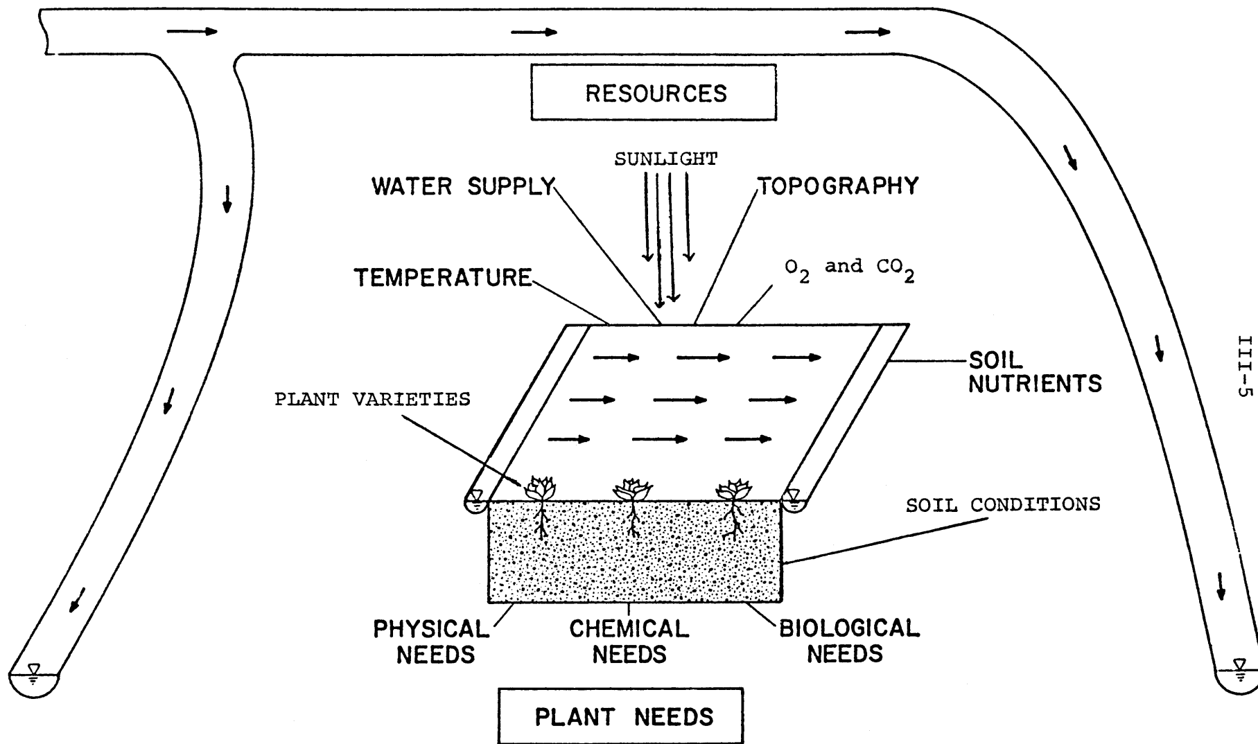
Figure 3.3. Idealized sketch of plant-soil components in a farm irrigation system.
