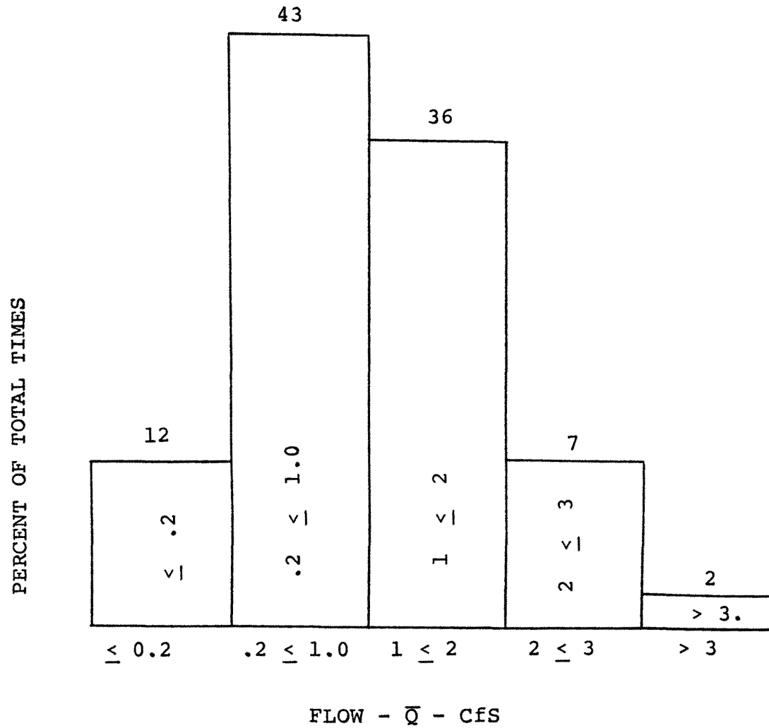
Figure 2.8. Seasonal frequency distribution of average flow rates at a field for a farm in Pakistan (Clyma et al., 1979).
