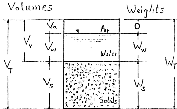
Figure 2.6. Definition of constants and some variables for the soil-air-water subsystem.
