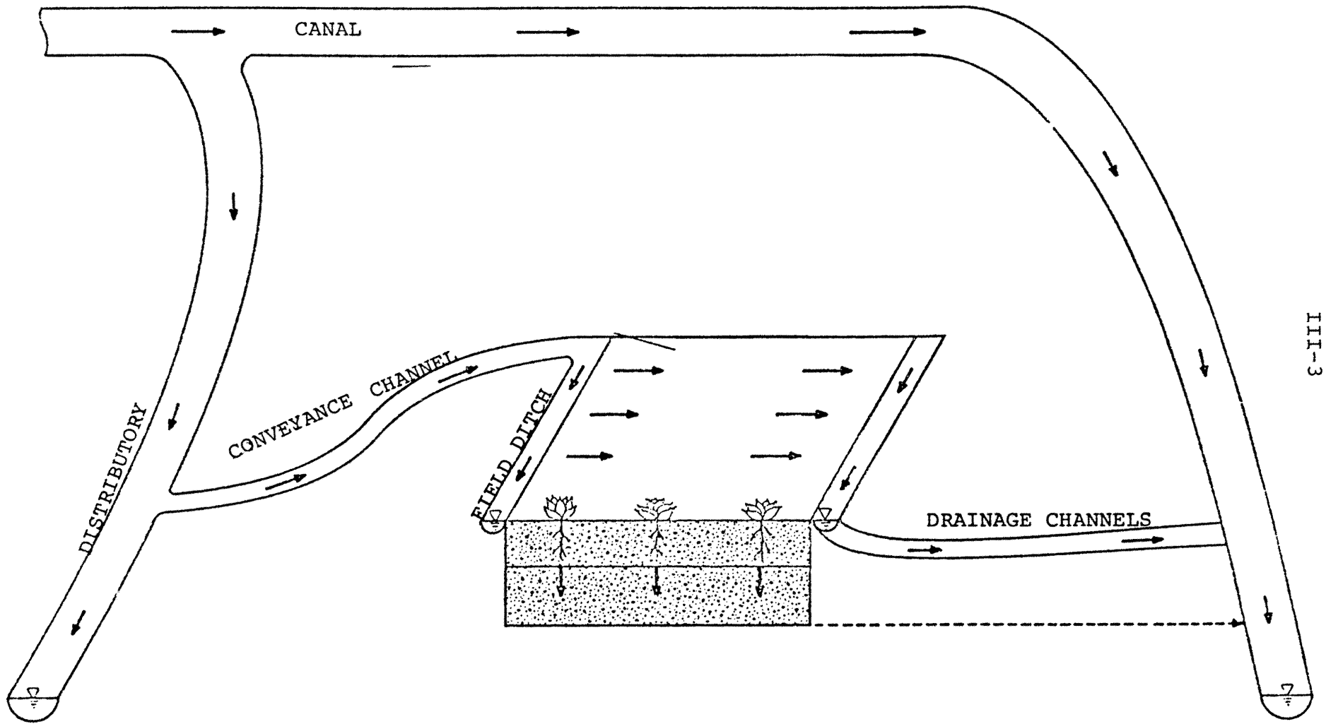
Figure 3.2. Idealized sketch of a farm irrigation system.
