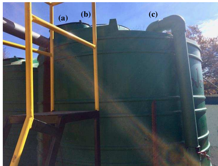
Figure 3.2: Photograph of the top of Tank 2; (a) access point, (b) chlorine drip dosage point, (c) vertical inlet
